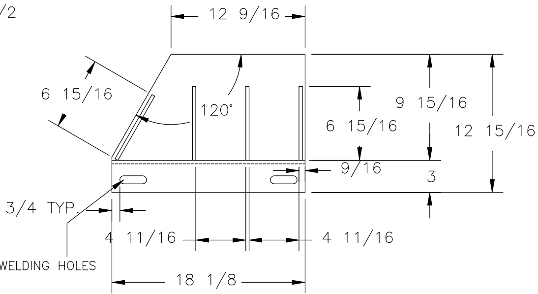
FRONT VIEW
