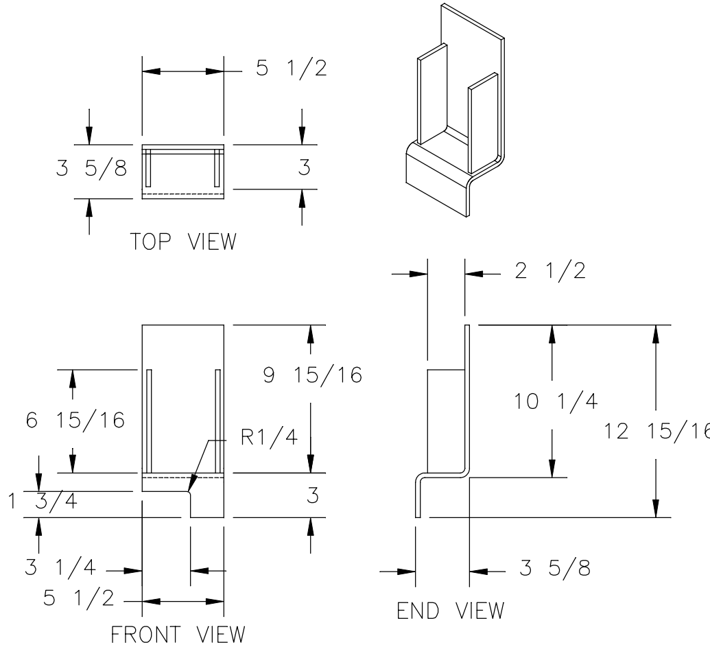
137990 SHORT UPPER RIGHT CAMBER BRACKET
