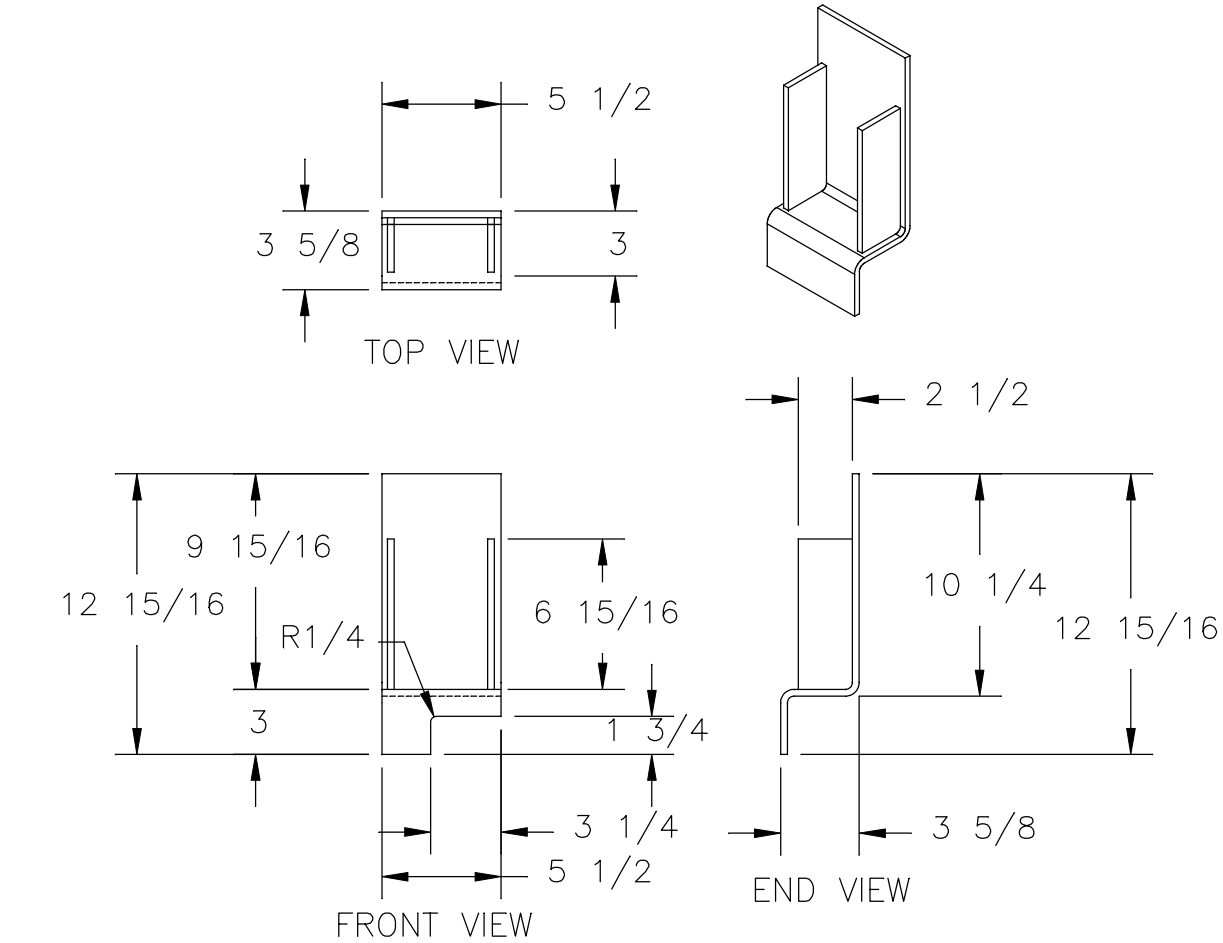
136205 SHORT UPPER LEFT CAMBER BRACKET
