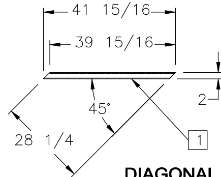
DIAGONAL DETAIL (3 REQ'D)
