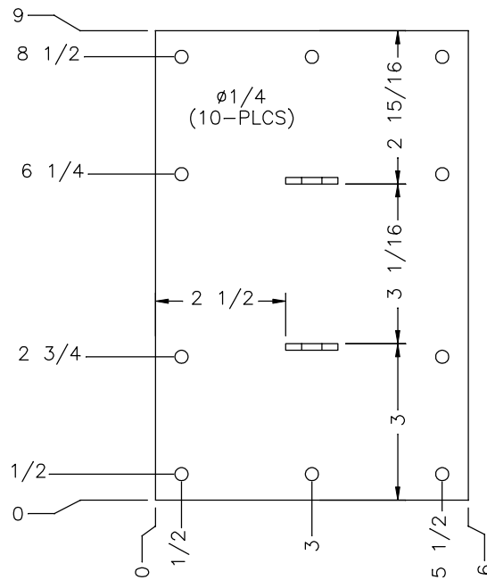
WALL PLATE (1/8" STEEL)
