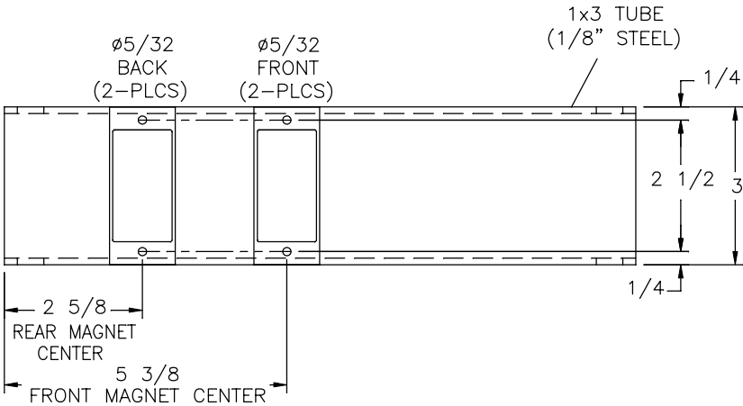
SWING ARM (FRONT VIEW)
