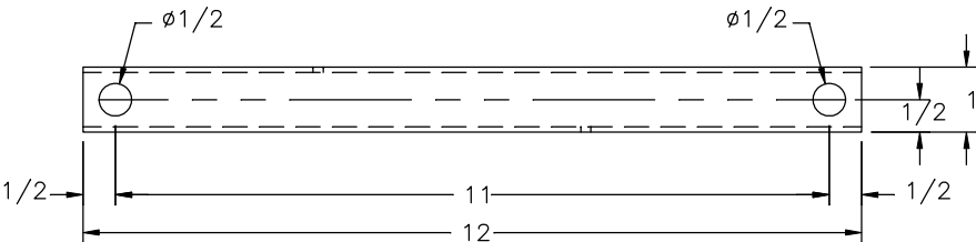
SWING ARM (TOP VIEW)
