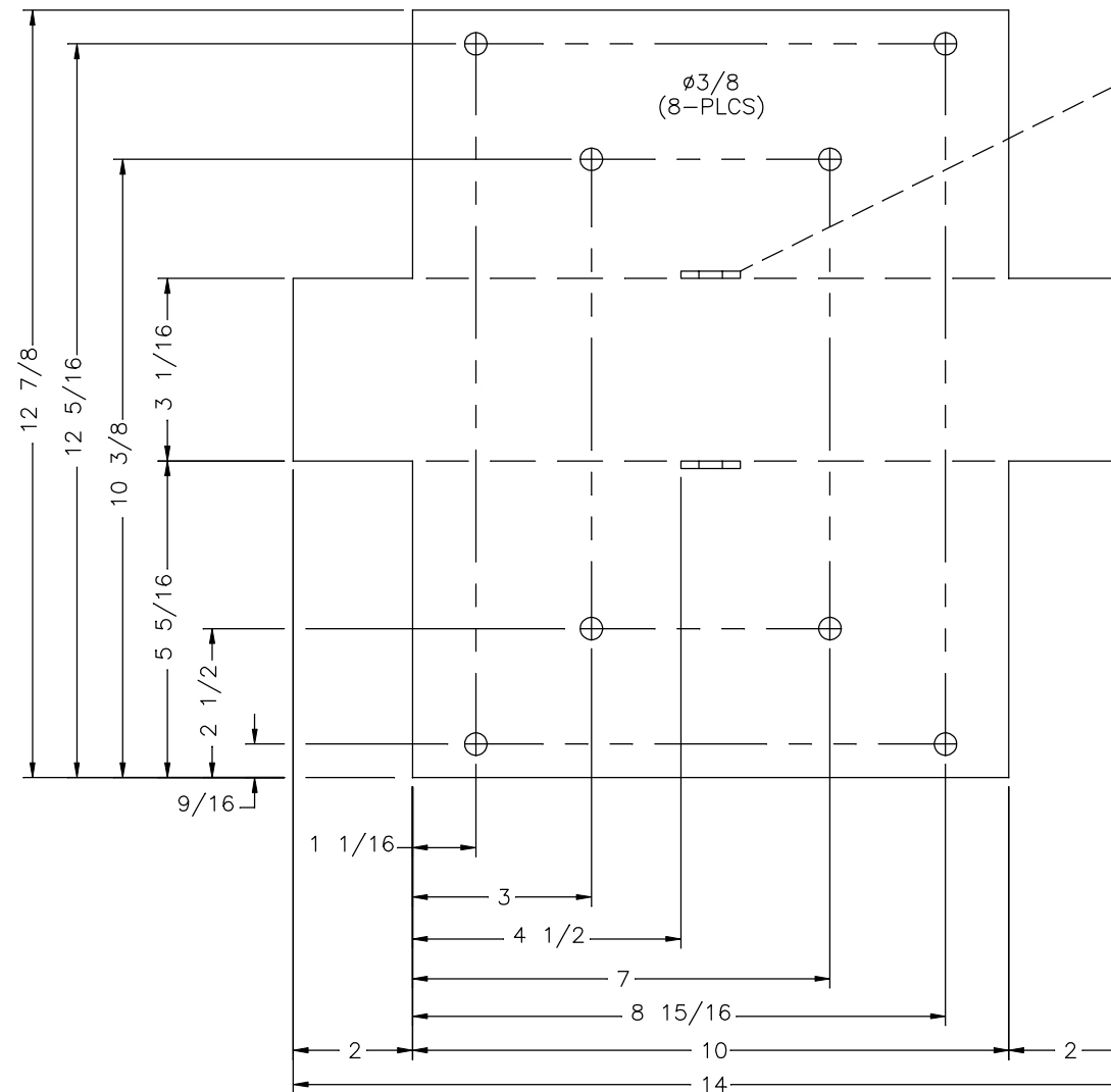
TV PLATE (1/8" STEEL)
