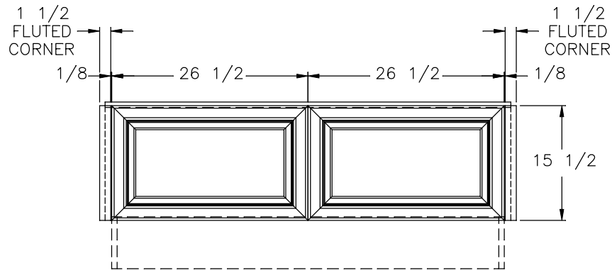
END (1—REQ'D)
