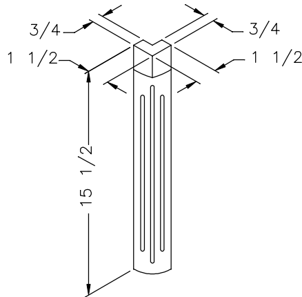
FLUTED CORNER
