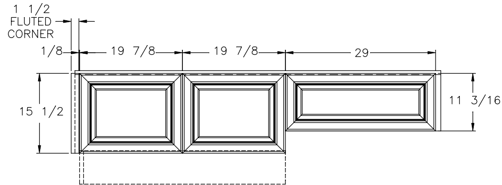
SIDES (2 SETS—REQ'D)
