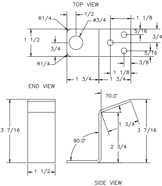
TAIL LIGHT BRACKET (TOP)
