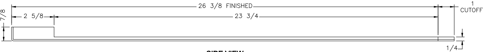
SIDE VIEW
