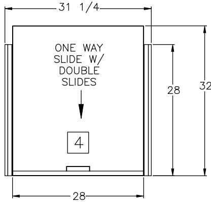
SMALL STORAGE TRAY ODS
