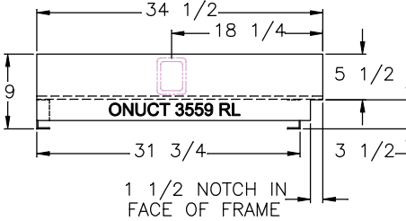
LARGE STORAGE TRAY
