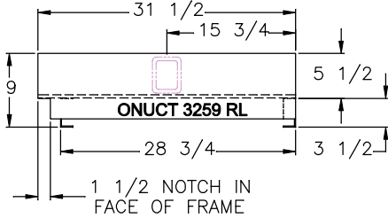
LARGE STORAGE TRAY
