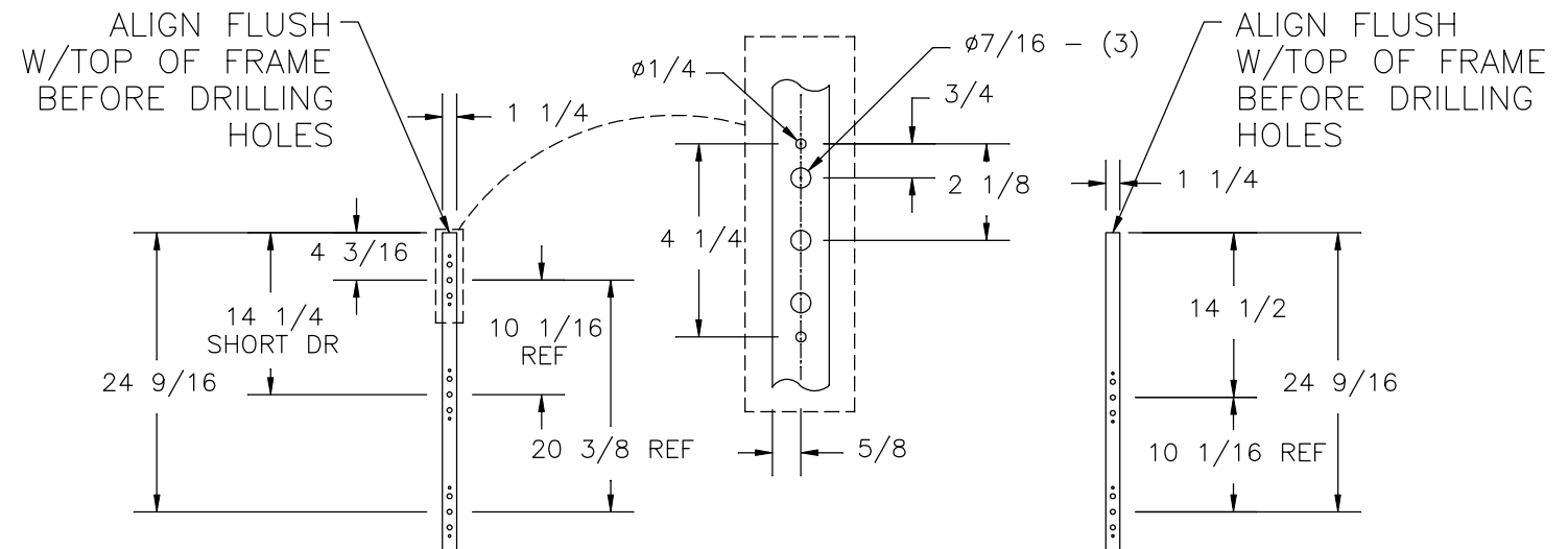
TEMPLATE FOR LOCATING HINGE HOLE LOCATIONS
