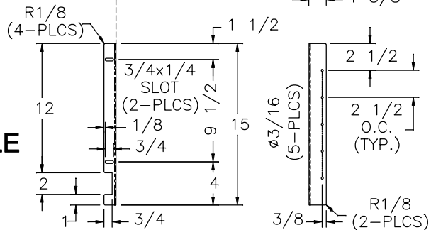
FRONT PANEL
