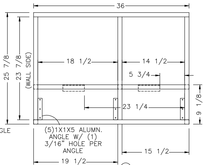
VIEW (C) BACK
