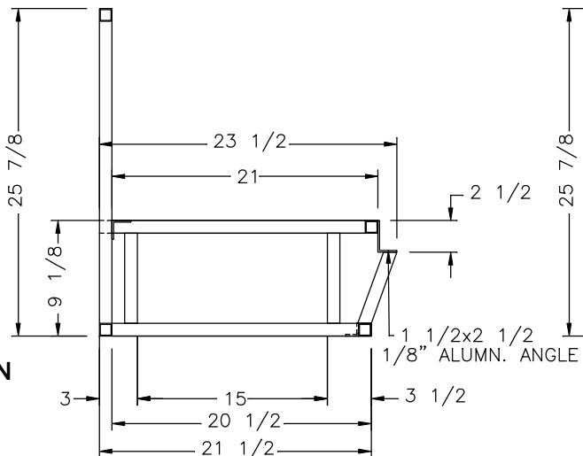
VIEW (B)
