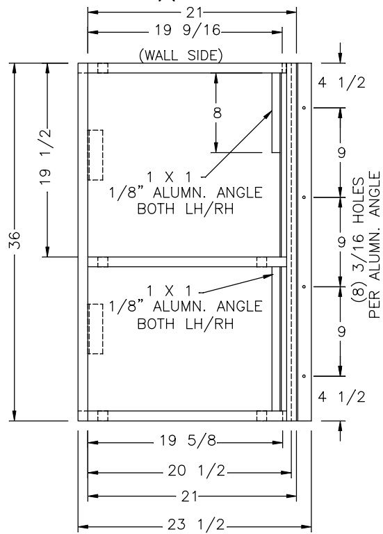
TOP VIEW (A) ASSEMBLED (LEFT HAND SHOWN) (RIGHT HAND OPPOSITE)
