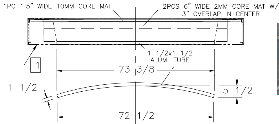
WIPER COVER ATTACHMENT BRACKETS
