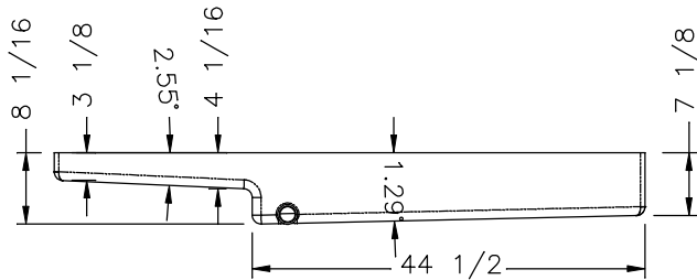
DISCHARGE END
