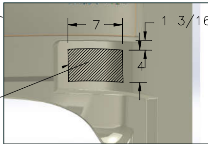
1/8 ALUM MIRROR BACKER CENTER
