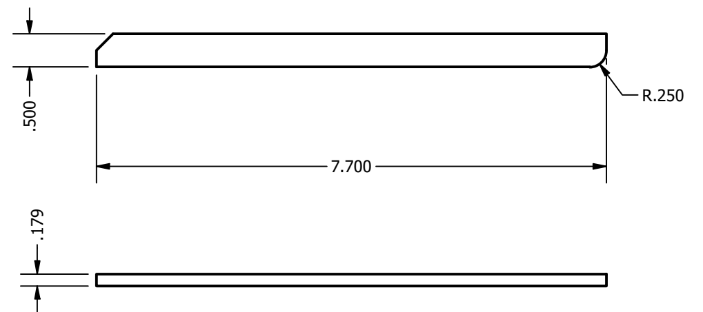
ITEM #3 MATERIAL: .179" (7 GA.) x .50" x 7.213" PLATE
