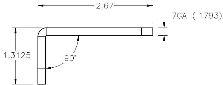
END VIEW AFTER FORMING
