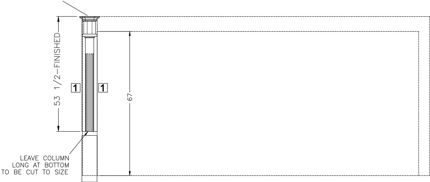
COLUMN HEADER C (SEE TYPICAL PRINT FOR DETAILS)
