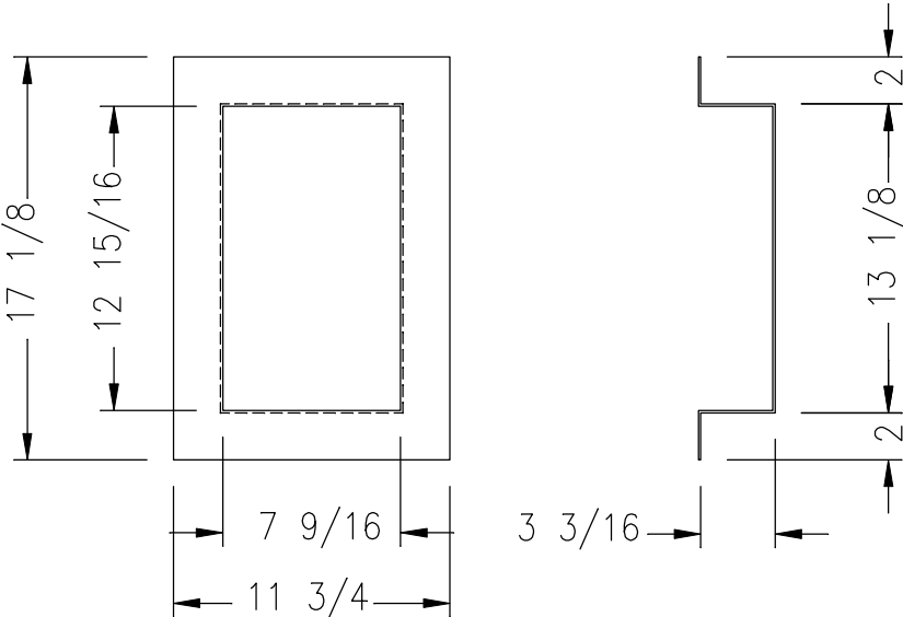
BLACK ABS BUCKET
