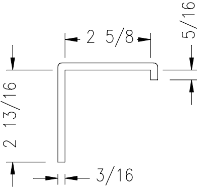
END VIEW (3x SCALE)
