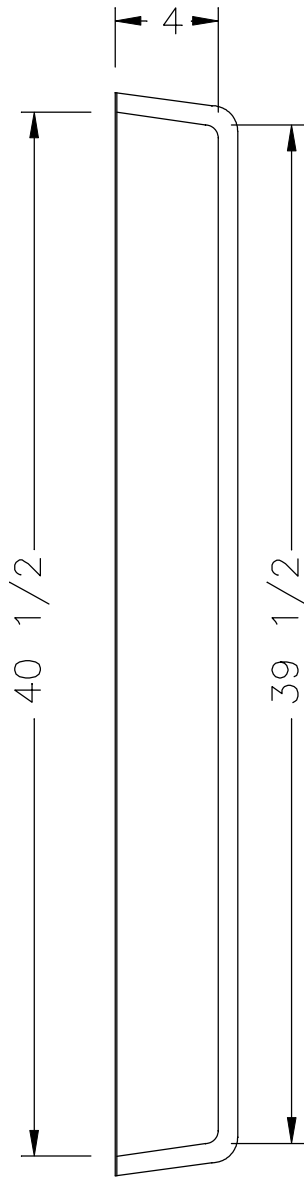
SIDE SECTION C
