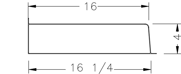
SIDE SECTION A
