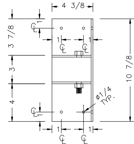
ARM MOUNT BRACKET FRONT
