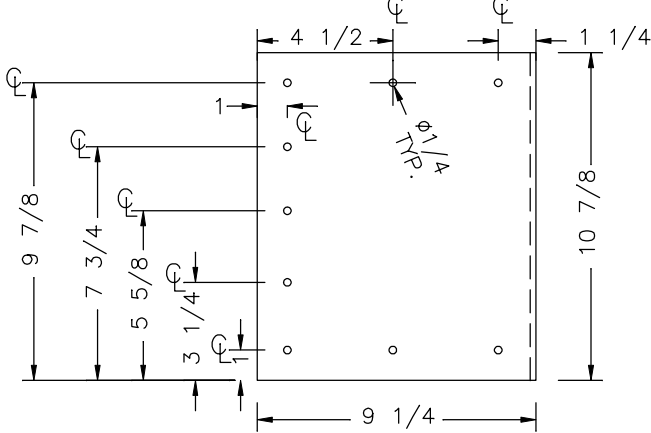
ARM MOUNT BRACKET SIDE
