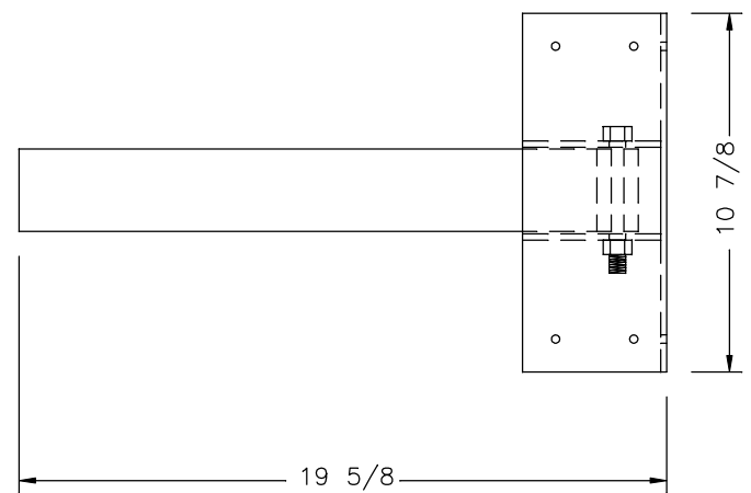
ASSEMBLED ARM FRONT
