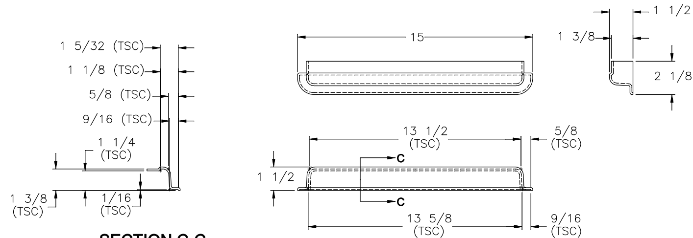
SECTION C-C TSC = THEORETICAL SHARP CORNER
