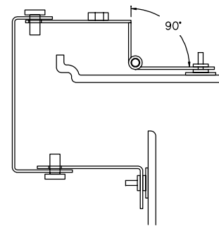
ASSEMBLED TOP VIEW DRIVER SIDE
