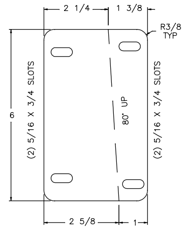
FLAT PATTERN
