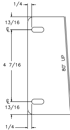
BENT VIEW
