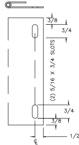
SECTION D
