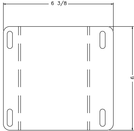
FLAT PATTERN
