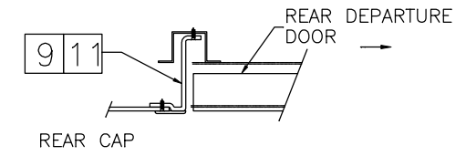
DOORSIDE TOP VIEW SCALE 2X
