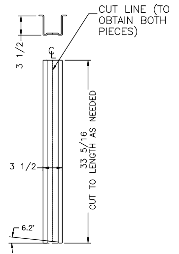
REAR DEPARTURE FILLER PANELS
