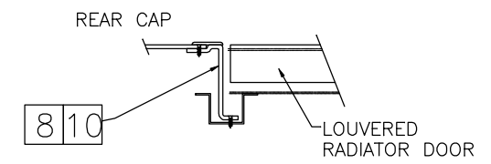
OFF DOORSIDE TOP VIEW SCALE 2X
