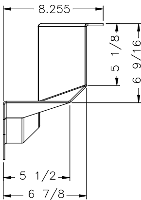
SIDE VIEW – LEFT
