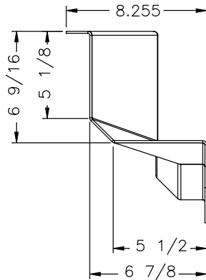
SIDE VIEW – LEFT
