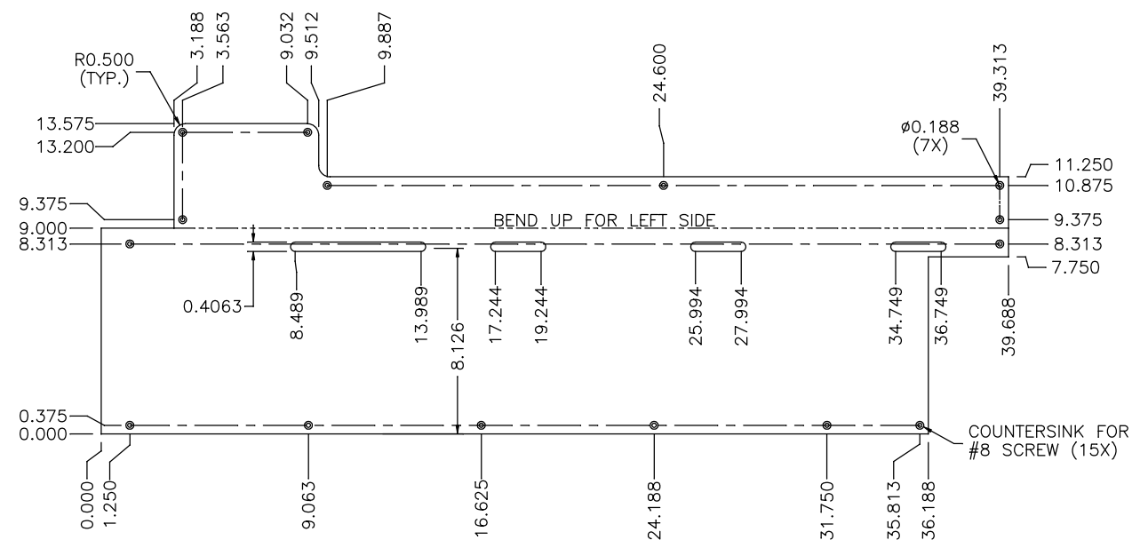
FLAT VIEW
