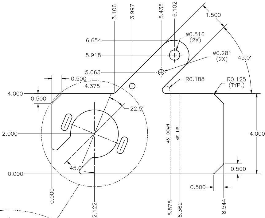
FLAT PATTERN
