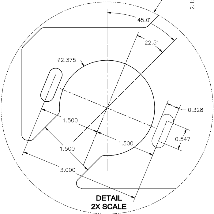
FLAT PATTERN
