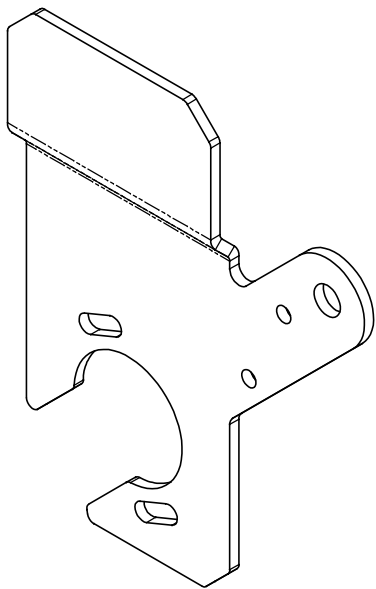
BENT ISO VIEW
