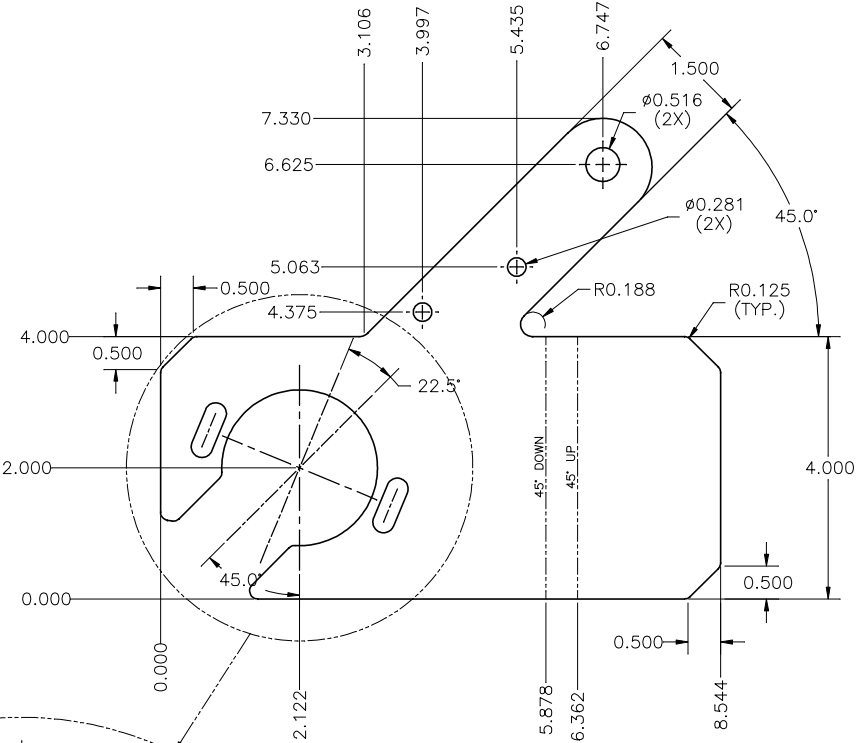
FLAT PATTERN
