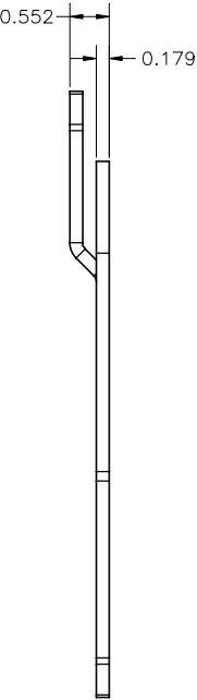
BENT END VIEW
