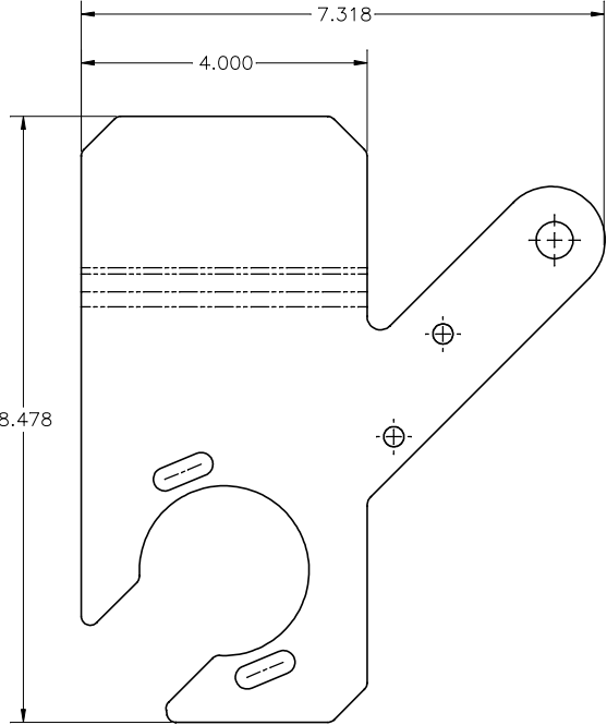
BENT SIDE VIEW
