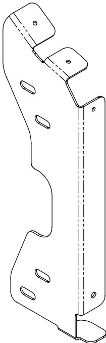
ISO VIEW
