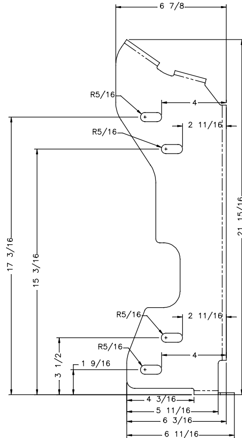
SIDE VIEW
