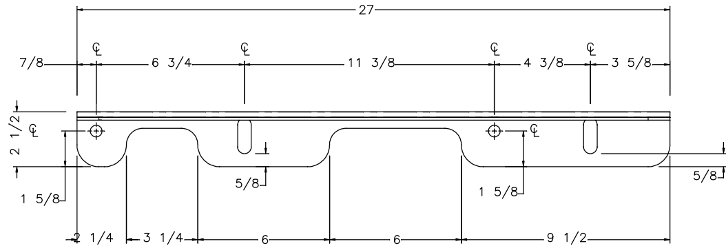
TOP VIEW
