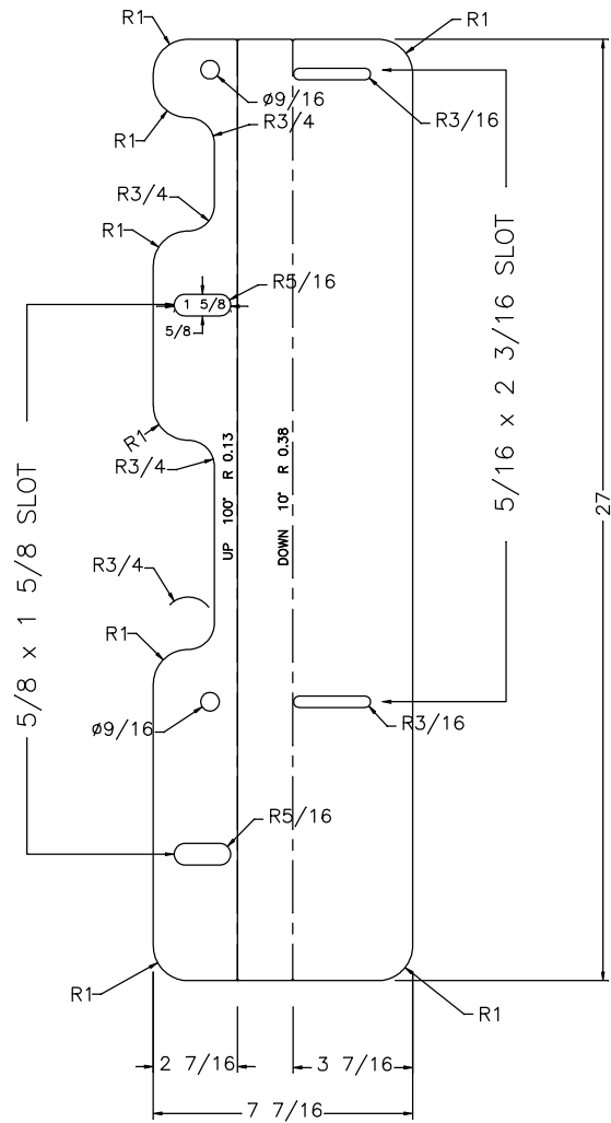
FLAT PATTERN
