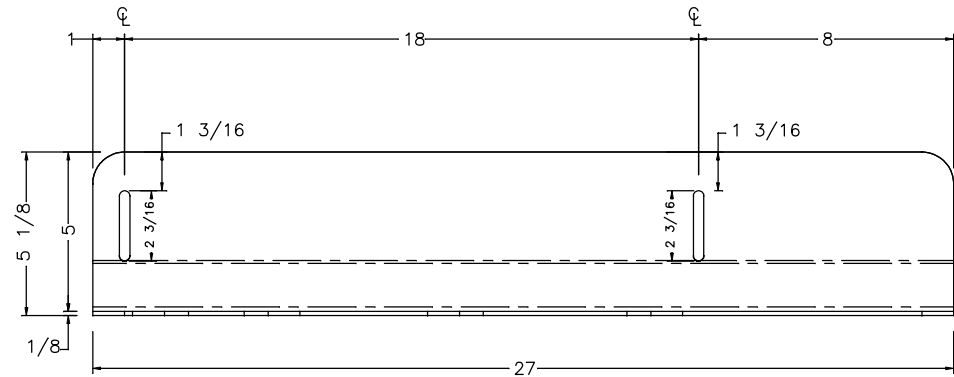
FRONT VIEW
