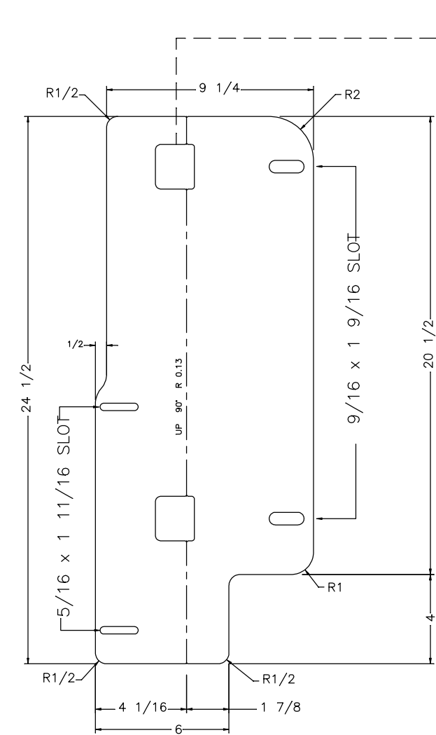
FLAT PATTERN
