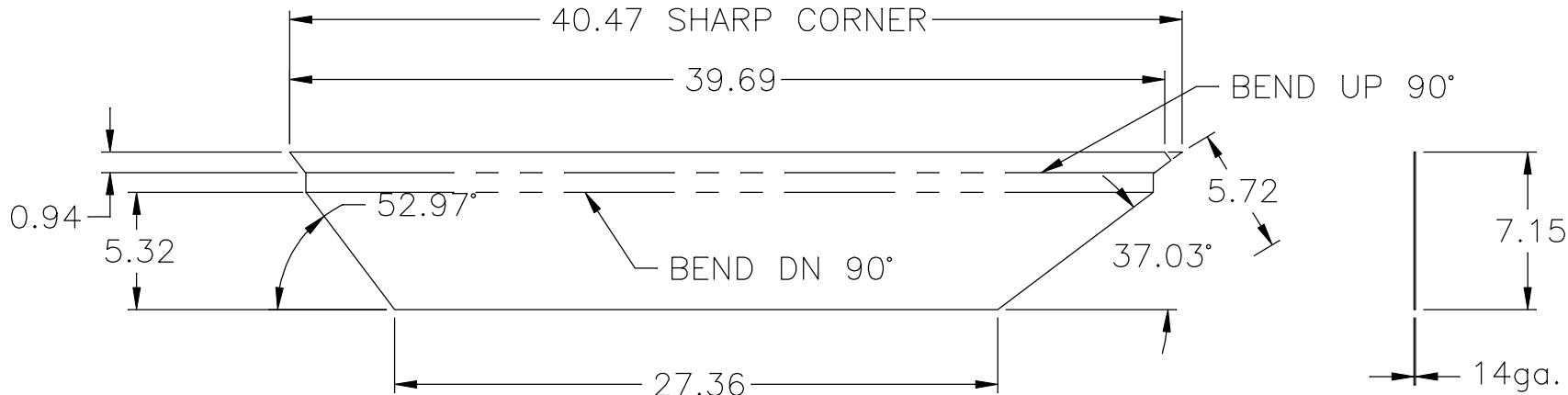
PART B FLAT PATTERN (2) REQ'D.
