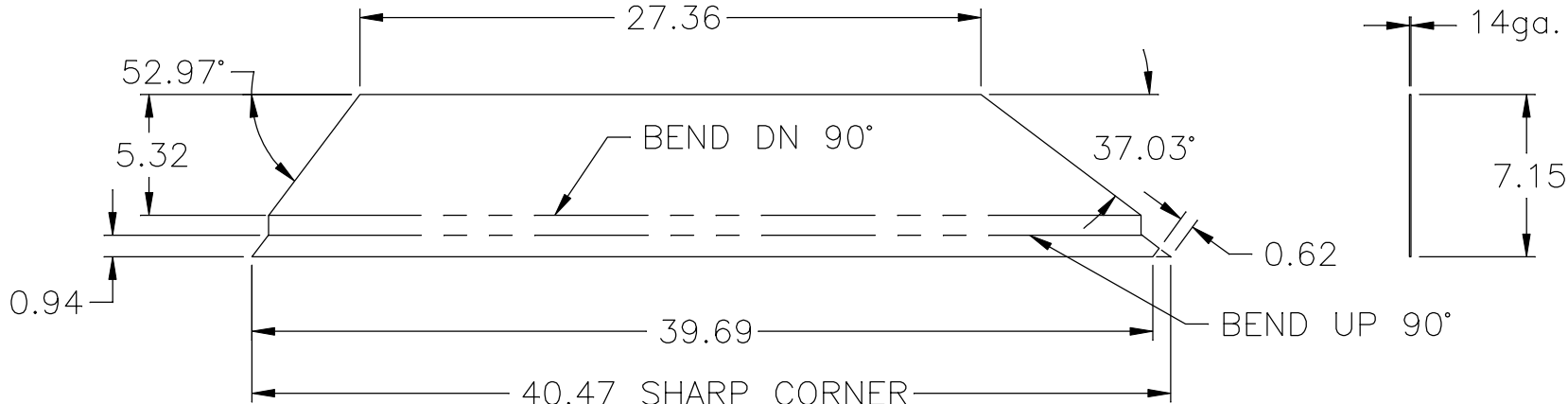
PART A FLAT PATTERN (2) REQ'D.
