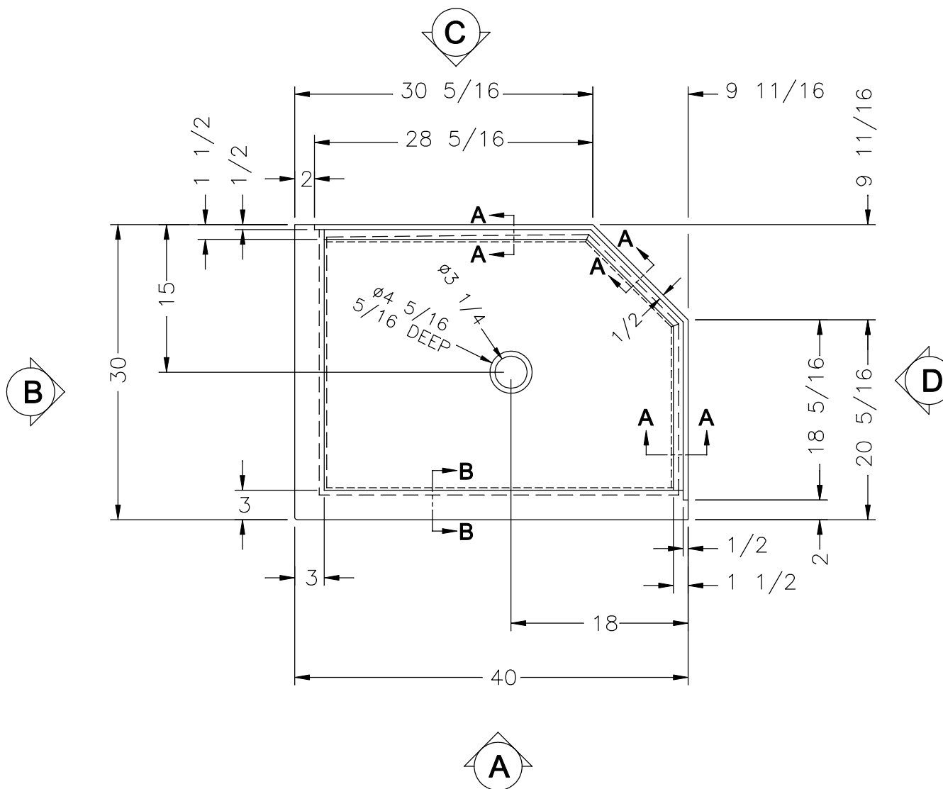
PLAN VIEW
