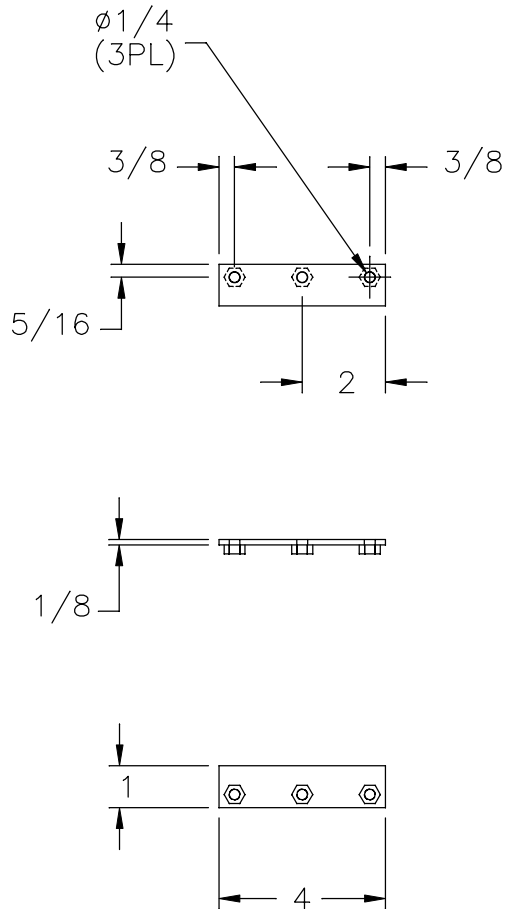
TOP PLATE
