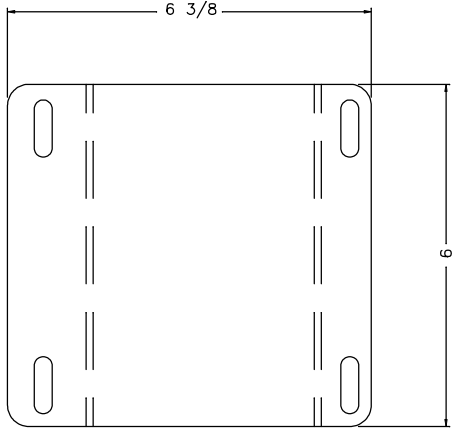
FLAT PATTERN
