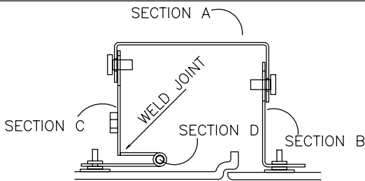
ASSEMBLED TOP VIEW PASSENGER SIDE
