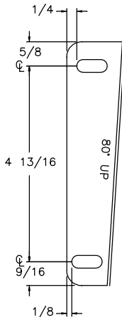
BENT VIEW
