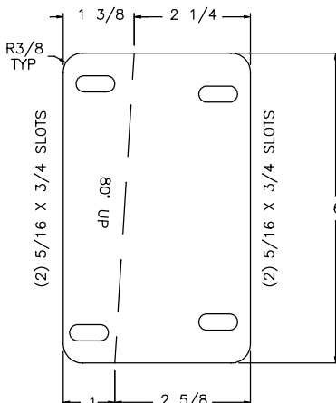
FLAT PATTERN
