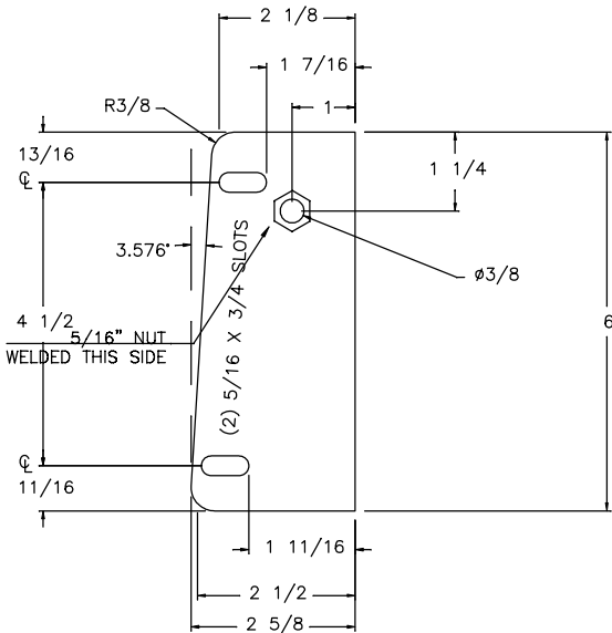
(PASSENGER SIDE SHOWN)
