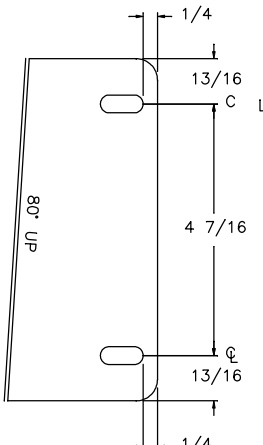
BENT VIEW
