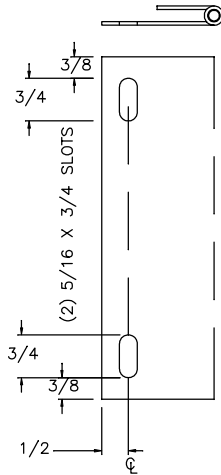
SECTION D
