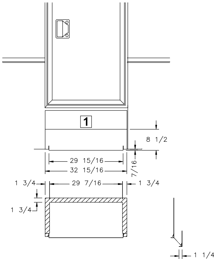
1 REAR VIEW NO TAPE ZONE
