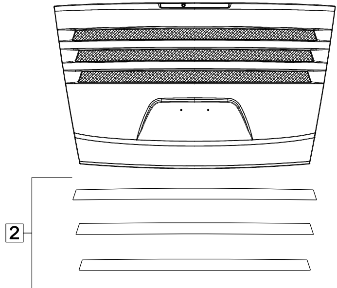
REAR DOOR TRIM (16ga Stainless Steel)
