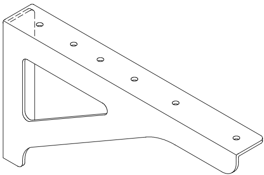
FINISHED PART ISO MATERIAL: 11 GA STEEL; BLACK POWDER COAT
