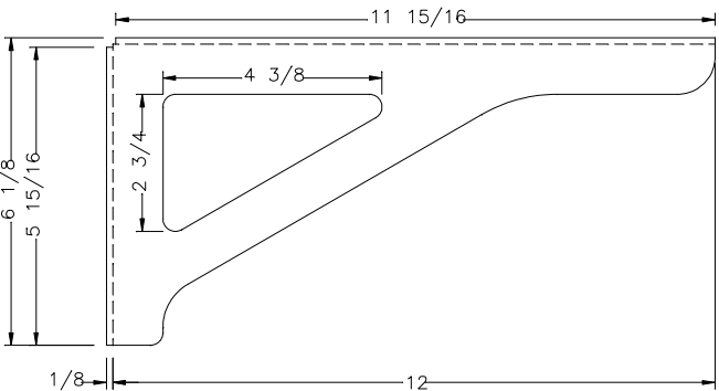
FINISHED FRONT VIEW
