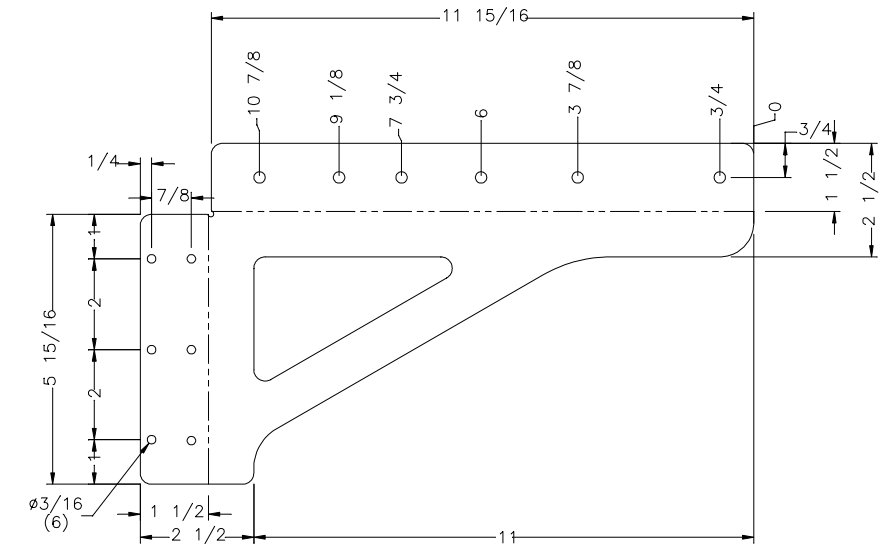
FLAT PART DIMENSIONS
