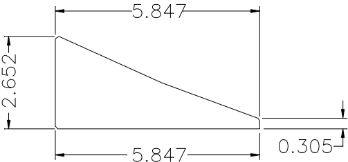
GUSSET 14 GA (.075")
