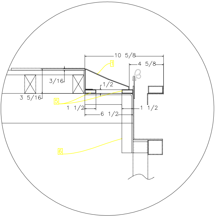
RAMP W/CARPET
