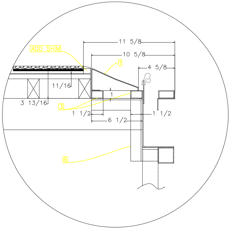
RAMP W/TILE
