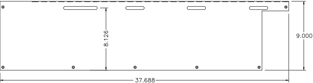
BENT BOTTOM VIEW
