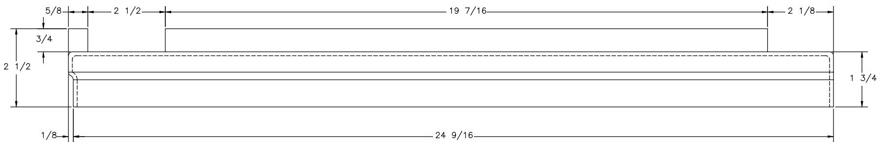
FRONT VIEW
