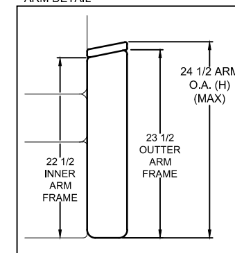
* ARM DETAIL
