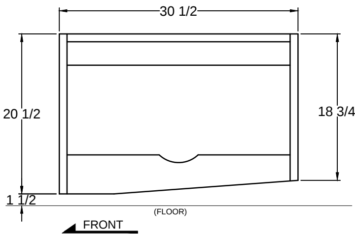
*ARM FRAME DETAIL (SIDE VIEW)
