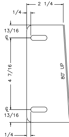
BENT VIEW
