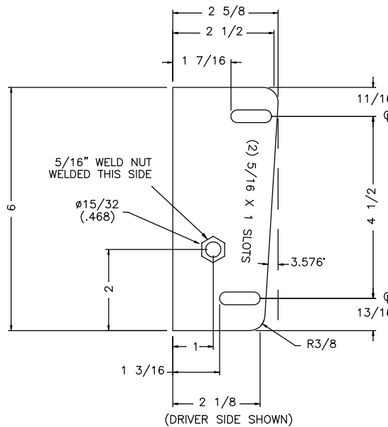
SECTION C
