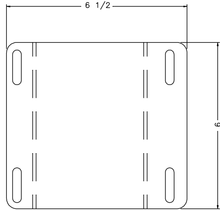
FLAT PATTERN
