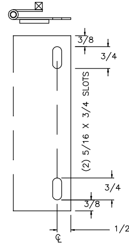
SECTION D
