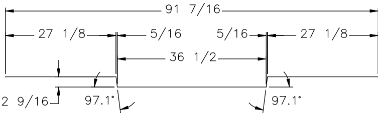
END VIEW
