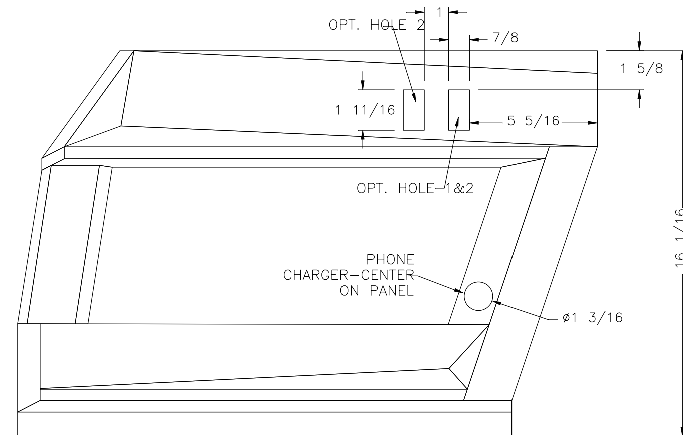
DRIVER FRONT VIEW
