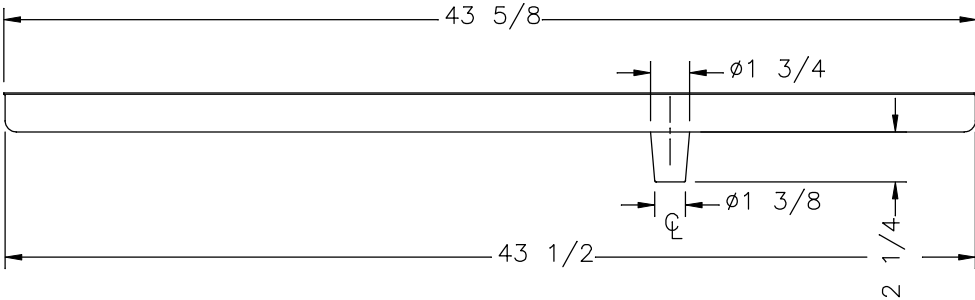
FRONT VIEW
