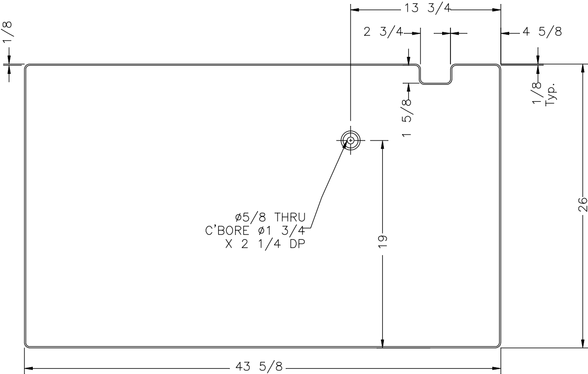
TOP VIEW
