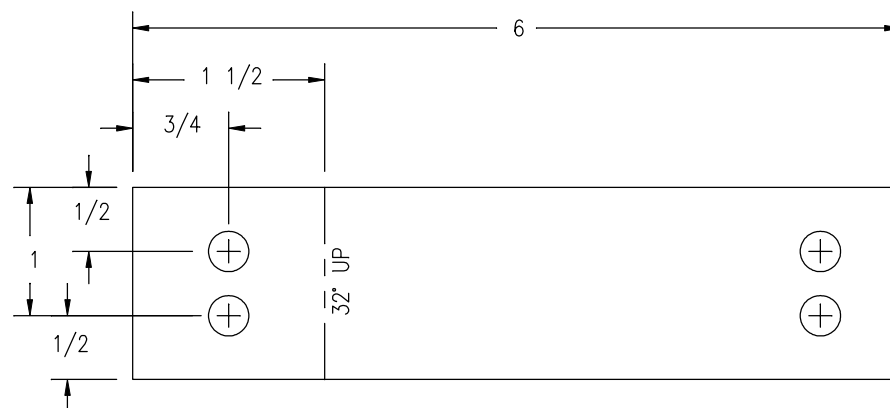
FLAT PATTERN
