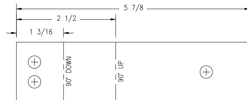
FLAT PATTERN
