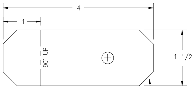
FLAT PATTERN
