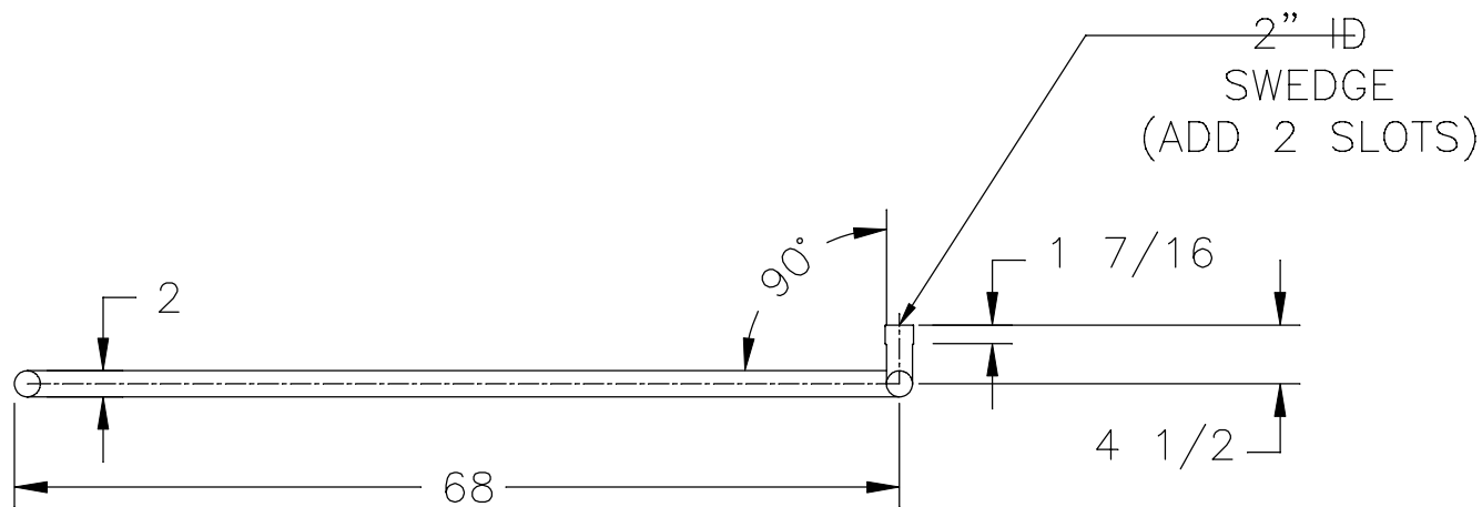
SIDE VIEW
