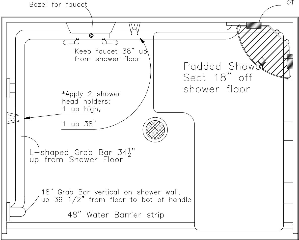
TOP VIEW OF SHOWER
