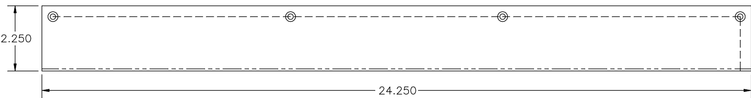
BENT FRONT VIEW
